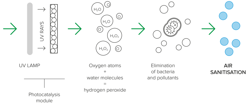
*Diagram of a generic photocatalysis process (by way of an example).
